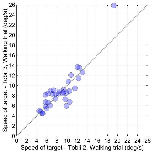
Fig. 12 Mean speed of the target in the camera image in the walking trials for the Tobii 2 and the Tobii 3. Each circular marker represents a participant ( n = 34 ). The dotted line represents the line of equality
