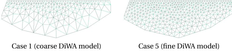
Figure 5.10: Two DiWA models with different grid resolutions
