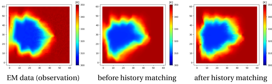
Figure 6.10: The history matching results of the reservoir temperature of the 4th layer of Egg model. The left figure shows the EM observation data of the "true" model. The middle and right figures are the results of realization #66 based on RML.
