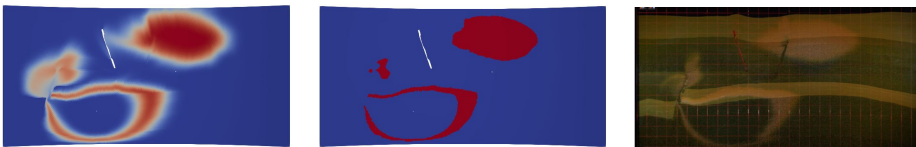
Figure 6.21: The tracer test results at the last time step. The left and middle figures are the results of numerical model response. The right figure is the experimental results.
