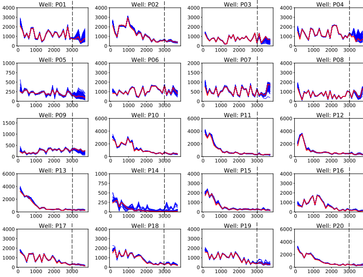
Figure 5.18: The oil rates of the 100 best-fit realizations (blue curves) and the observation data (red curves); the x-axis shows the production time (days), the y-axis shows the oil production rate ( \text{m}^3/\text{day} ); the mean error of training period and prediction period between these 100 realizations of DiWA model of Case 5 (fine model) and the observation data are 0.44% and 0.17%, respectively
