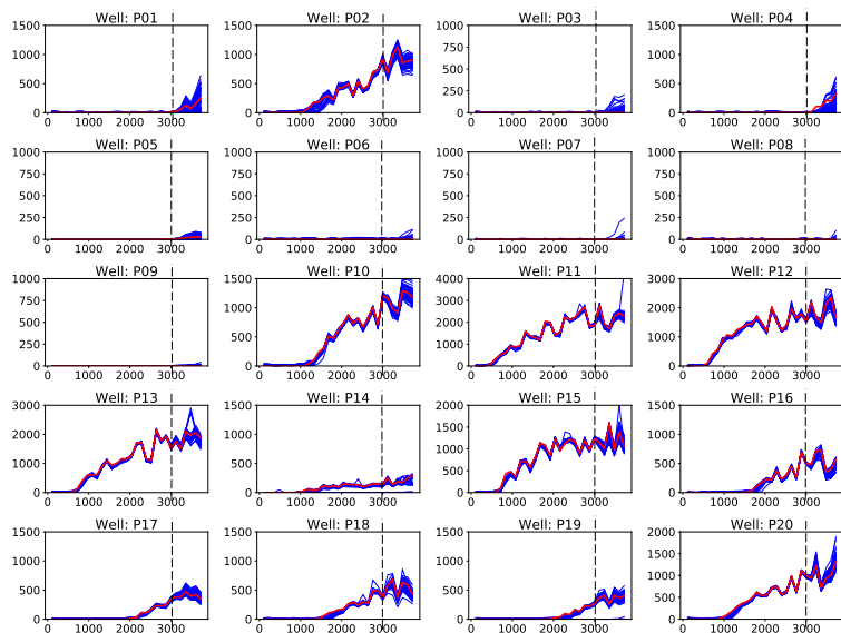
Figure 5.19: The water production rates of the 100 best-fit realizations (blue curves) and the observation data (red curves) for Case 5; the x-axis shows the production time (days), the y-axis shows the oil production rate ( \text{m}^3/\text{day} )
