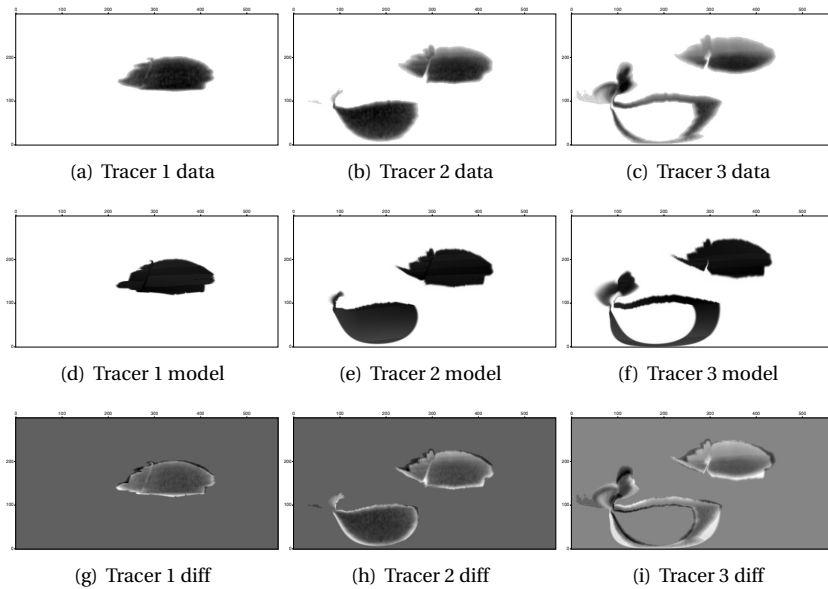
Figure 6.18: Tracer data image and associated MAP forward models. Greyscale is [0,1]=[white,black] .
