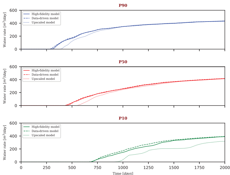
Figure 5.4: P10, P50 and P90 quantile response of the high-fidelity (reference), DiWA data-driven, and upscaled models for 100 FLUMY realizations.
