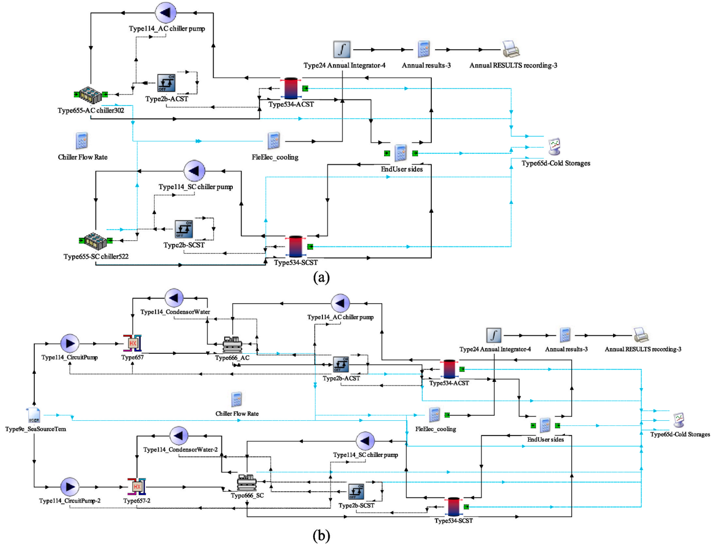
Fig. 3. Systematic configuration of cooling systems in TRNSYS 18: (a) air-cooled chiller; (b) water-cooled chiller.
