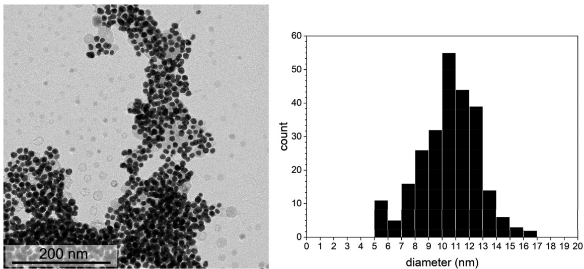
Figure 6: (Left) TEM image of mercury-spiked AuNPs [Method (B2)], and (right) the corresponding histogram of their diameters. Several spherical AuNPs were visible with an average size of 10.5 \pm 2.2 nm as assessed from 253 independent measurements.
