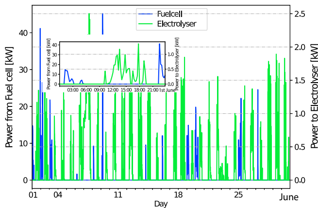
Fig. 9. Electrical power injection from the fuel cell and electrical power taken by the electrolyser in June
