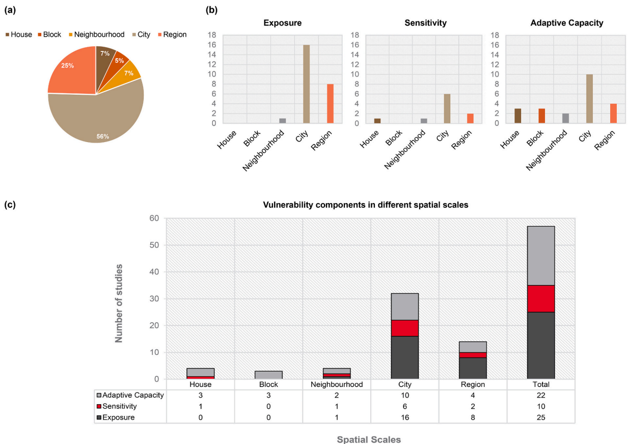
Fig. 7. (a) Share of studies per spatial scales (n = 57); (b) Studies related to each vulnerability components across spatial scales; (c) Overall distribution of studies in different spatial scales incorporating all three vulnerability components reveals an emphasis on macro-level (city, region) investigations while micro-level (house, block, neighbourhood) studies are limited.
