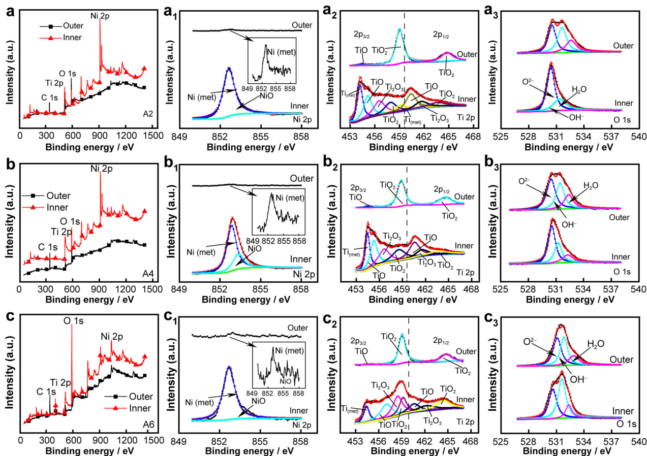
Fig. 9 XPS peaks comparison of L-PBF NiTi after being immersed in artificial saliva for 168 h: a–a 3 : A2 ( 56 \text{ J} \cdot \text{mm}^{-3} ); b–b 3 : A4 ( 87 \text{ J} \cdot \text{mm}^{-3} ) and c–c 3 : A6 ( 60 \text{ J} \cdot \text{mm}^{-3} )
