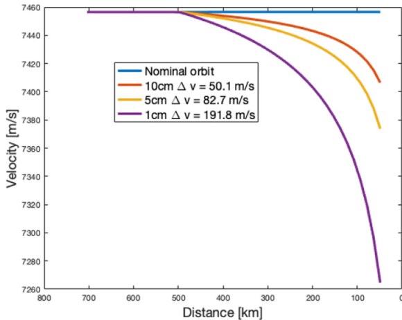
Fig. 3. Induced velocity change on objects with different size for head-on geometry at 800 km. X-axis expresses the relative distance between the debris object and the laser system during the interaction.
