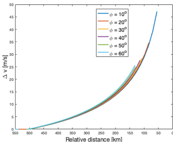
Fig. 4. \Delta v on 10 cm debris objects from a non-zero azimuth angle.
