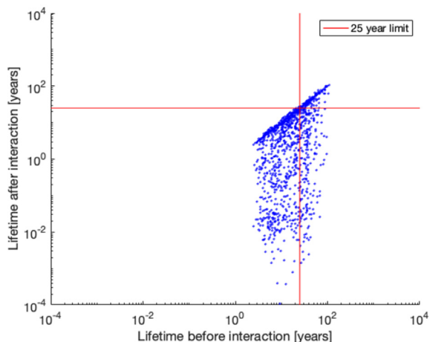
Fig. 8. Cumulative decrease in lifetime on the 1739 different encountered objects.
