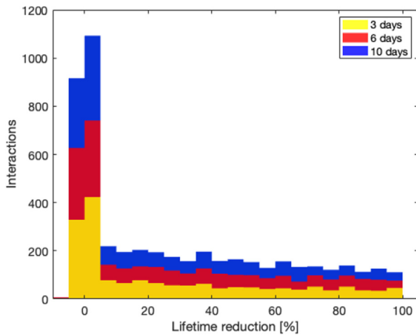
Fig. 6. Lifetime reduction for all 5000 interactions.
