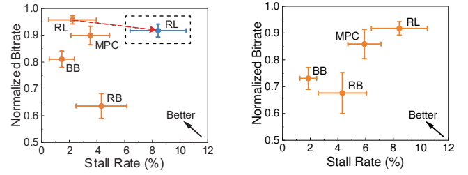
Fig. 4. QoE factors of ABR algorithms under 4G & 5G network conditions.
