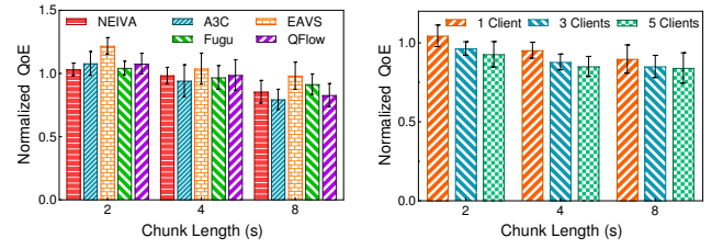
(a) Various methods.
