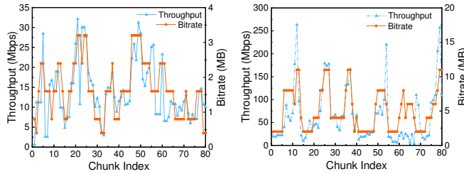
(a) PPO for 4G trace.
