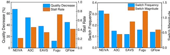
(a) Video quality v.s. stall rate.
