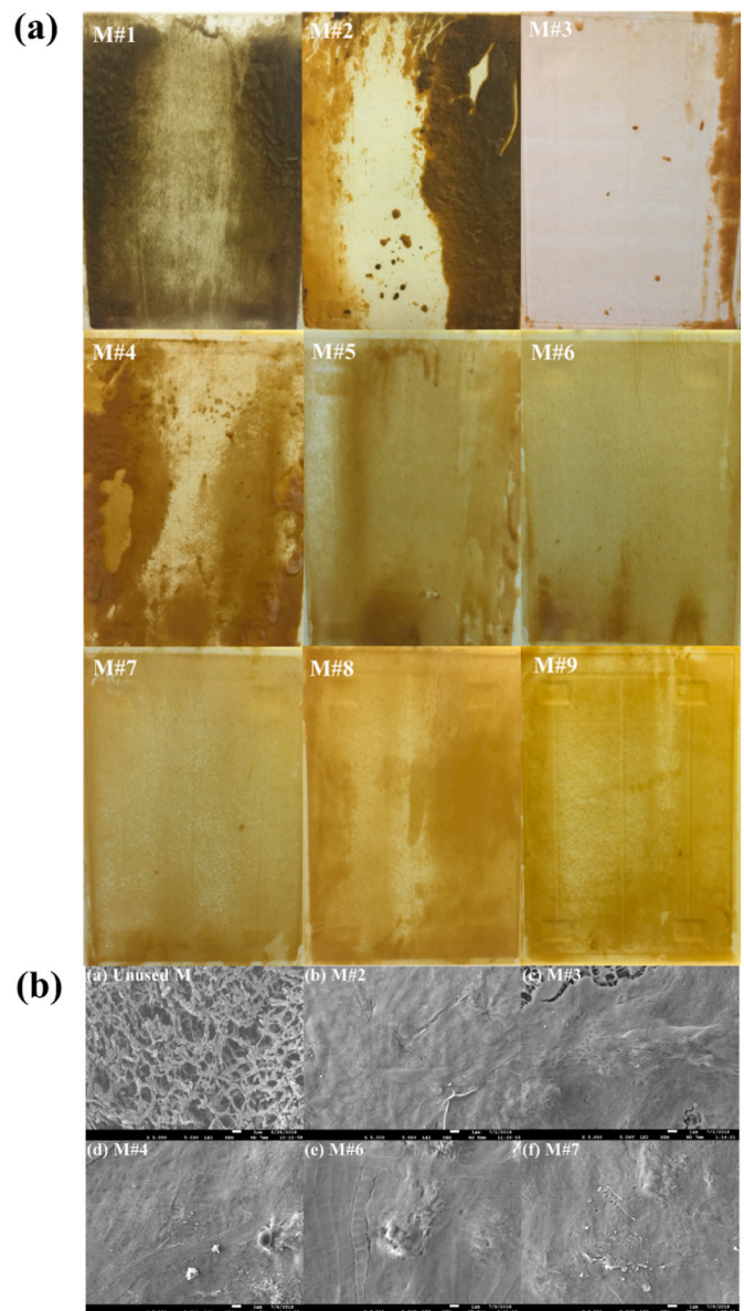
Fig. 5. (A) Images of the fouled membranes for the membrane bioreactor equipped with bubble diffusers (M#1 to M#3) and with the supersaturated dissolved oxygen unit (M#4 to M#9); and (b) Scanning electron microscope images of the fouled membranes: Unused membrane (a), M#2 (b), M#3 (c), M#4 (d), M#6 (e), and M#7 (f).
