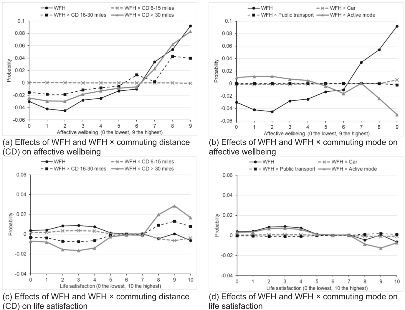
Fig. 4. Marginal effects of switching to WFH and the interaction with pre-pandemic commuting behaviours on SWB outcomes.
