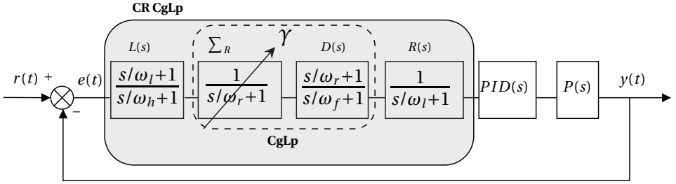
Figure 6.7: The control loop used for precision motion control using CR CgLp. P(s) is the plant. PID(s) = k_p(1 + \omega_i/s) \left( \frac{s/\omega_d + 1}{s/\omega_t + 1} \right) .
