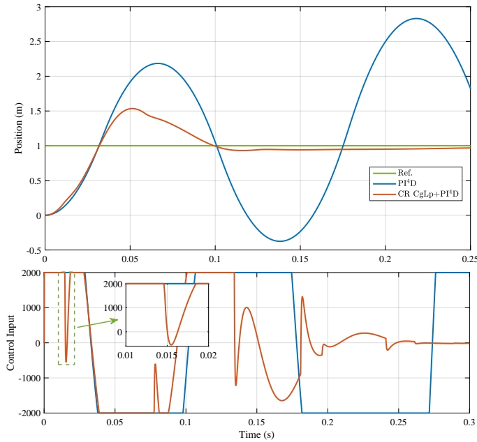
Figure 7.8: Step response of CR CgLp+PI 4 D and PI 4 D. The controllers are the same as in Fig. 7.7 and the control input signal is saturated at 2000 level.
