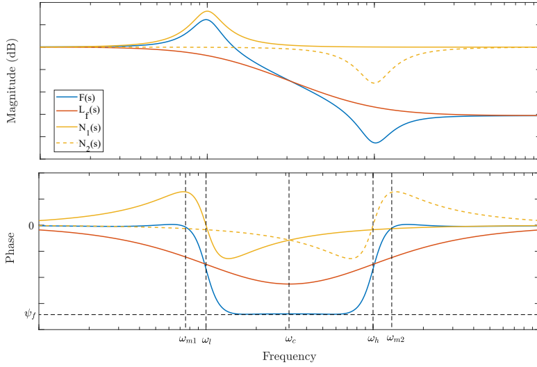
Figure 4.8: Bode diagram of the composition of F(s) .
