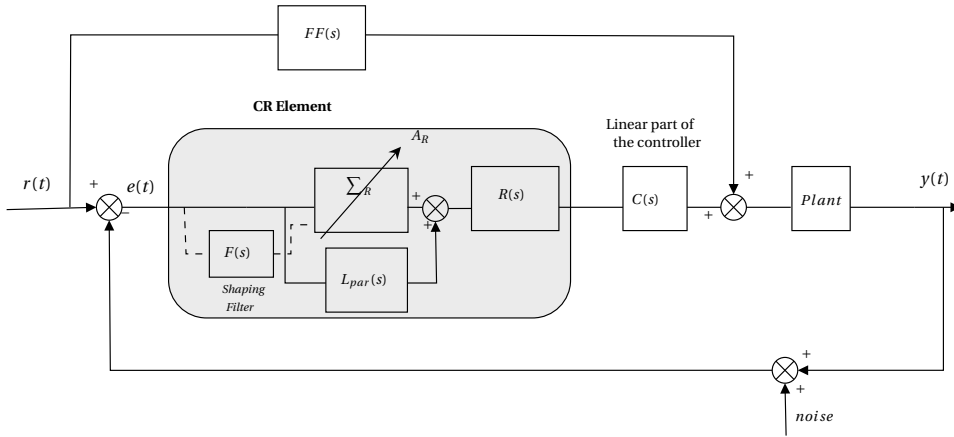
Figure 1.8: Closed-loop architecture containing parallel CR architecture.
