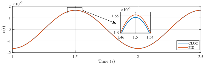
Figure 5.9: Sinusoidal tracking error of CLOC and PID for r(t) = \sin(2\pi t) .
