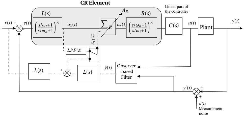
Figure 9.11: The concept of using higher-order lead element in CR CgP to have less amplification of high-frequency content of noisy reset signal. LPF(s) = 1/(s/\omega_{CO} + 1) .
