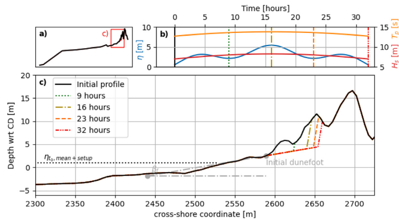
Fig. 13. Results of the wave impact model presented in Larson et al. (2004a) (c) on the Meijndel transect (a). The storm hydrograph is displayed in (b).
