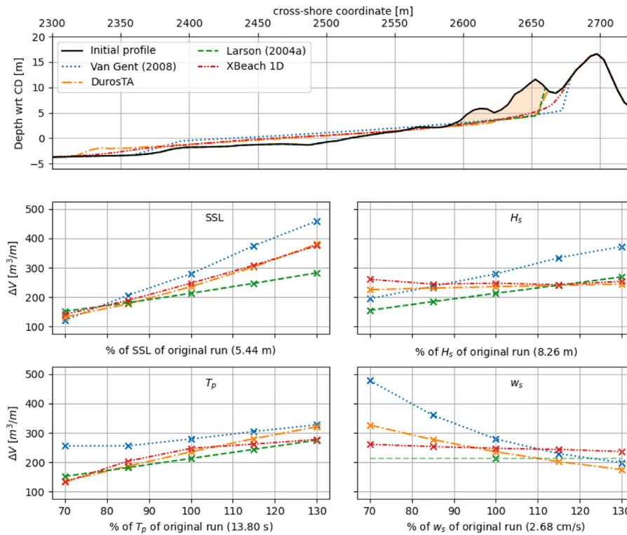
Fig. 16. Model sensitivities to SSL, H_s , T_p , and w_s . The upper panel displays the final profile of each model for the Meijendel transect when run with the standard hydrodynamic conditions. The lower panels display the eroded volume \Delta V in [m³/m], shoreward of x = 2300 m. The total eroded volume of DurosTA is displayed in yellow in the upper panel.
