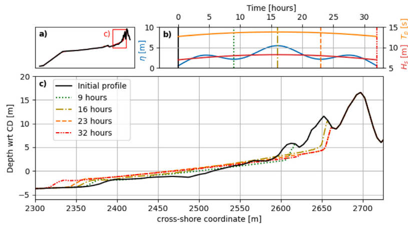
Fig. 12. Results of the DurosTA model of Steetzel (1993) with standard settings on the Meijndel transect. The storm conditions vary in time as displayed in (b), and the coloured profiles in (c) correspond to the moments in time displayed with vertical lines in (b). The total storm duration is 32 h.
