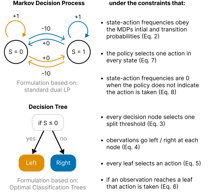
Figure 2: Overview of OMDT’s formulation. We maximize the discounted return in an MDP under the constraint that the policy is represented by a size-limited decision tree.
