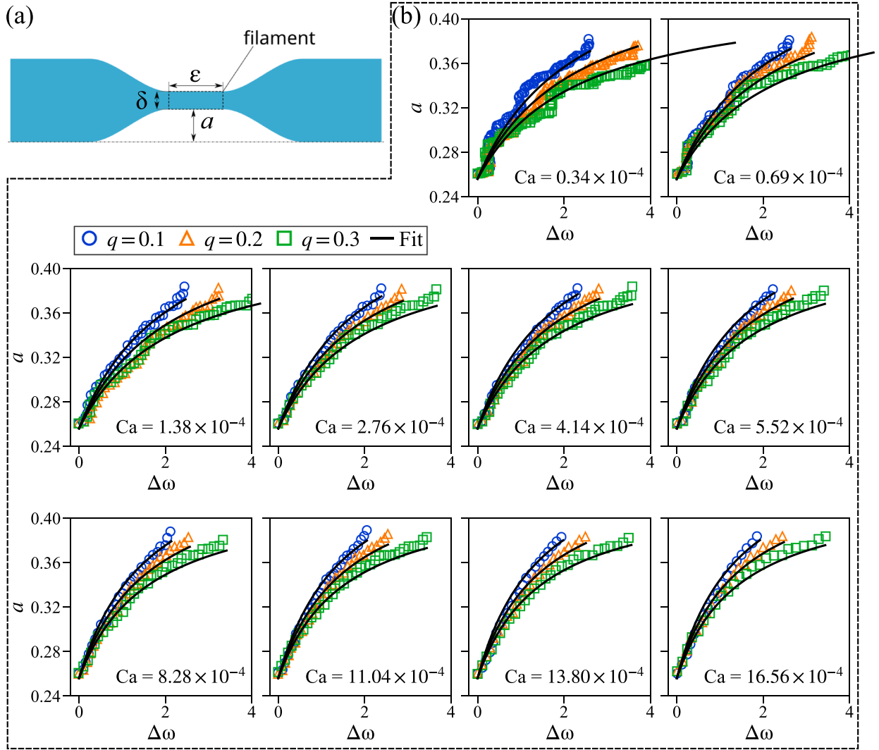
Fig. 9. (a) In the upper regime a > 0.26 , the increase in filament length \epsilon is faster than the thinning of filament width \delta . (b) Kinematics of the filamenting stage. Points are the experimental data for different values of q . The solid lines are the fitting results of Eq. (20) with fitting parameters. \epsilon_0 = 1.32 + 2.51 \times 10^{-4} (1.63 \times 10^{-4} + Ca)^{-1} . Graphs without a y-axis label and numbers have their y-axis shared with the figure on their left. Measurements were taken in the device with W/H = 4.07 .
