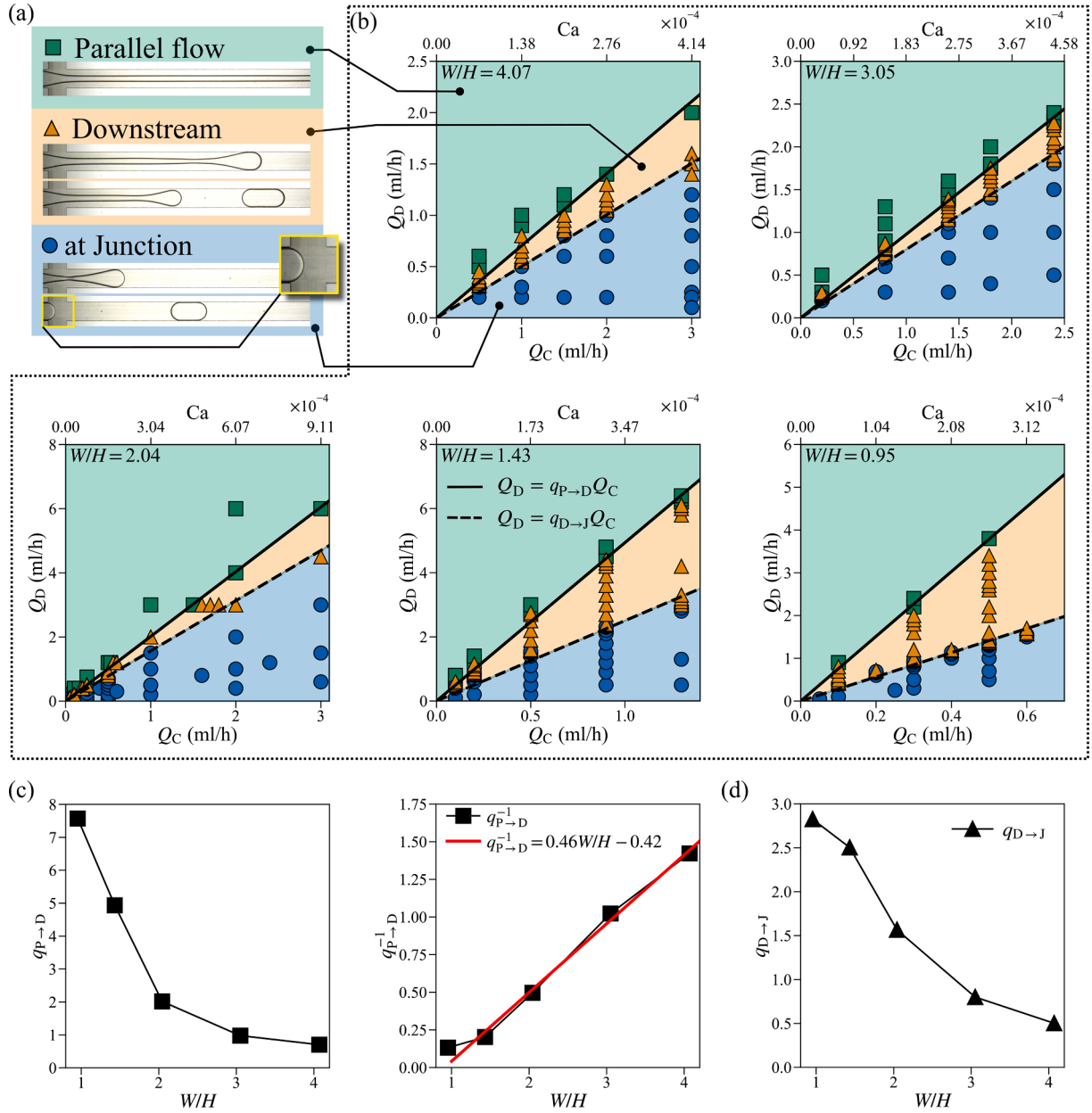
Fig. 10. Operating range for the three types of flow observed in the cross-junction devices with rectangular channels of different channel aspect ratios. (a) Experimental images showing the three observed flow types: formation of stable thread along the main channel – “Parallel Flow”, formation of droplets downstream of the junction – “Downstream”, and formation of droplets at the junction – “at Junction”. For both droplet flow types, two images represent the forming droplet before (top) and after (bottom) pinch-off. For droplet formation at the junction, the interface fully recedes to the junction after pinch-off, as shown in the close-up image. (b) Maps illustrating the operating range for parallel flow (green squares), the formation of droplets downstream (yellow triangles) and at the junction (blue circles) for devices with different W/H . For each map, the transition between parallel flow and droplet formation downstream of the junction is shown by the solid black line ( Q_D = q_{P→D} Q_C ). The transition between the two droplet formation types is shown by the dashed black line ( Q_D = q_{D→J} Q_C ). (c) The influence of the channel aspect ratio on q_{P→D} (left) shows that the inverse of q_{P→D} is proportional to the aspect ratio (right). (d) Influence of the channel aspect ratio on the flow rate ratio q_{D→J} that demarcates the operating range for the flow type central to this work: droplet formation at the junction. Images were taken from experiment in the device W/H = 4.07 . (For interpretation of the references to colour in this figure legend, the reader is referred to the web version of this article.)
