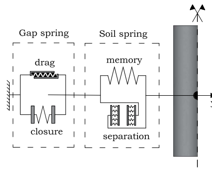
Fig. 12. 1D modeling scheme for the simulation of cyclic hysteresis with ratcheting control and pile–soil gapping, left side of the pile only; a similar scheme is also applied to the right side (adapted from Kementzetzidis et al. 2022).
