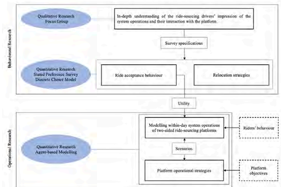
Figure 1-3: Research approach
