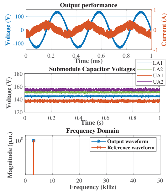
Fig. 10: Sinusoidal waveform with 3 kHz Frequency
