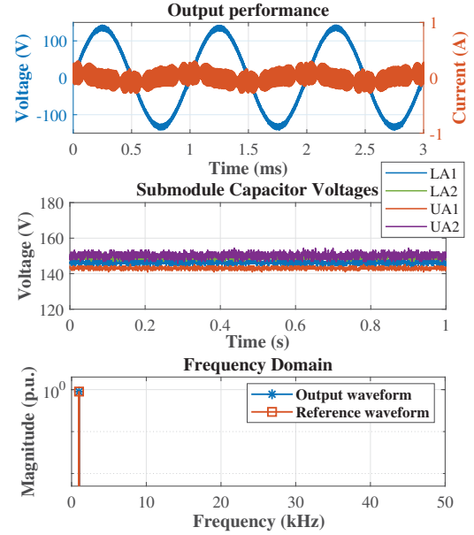
Fig. 9: Sinusoidal waveform with 1 kHz Frequency
