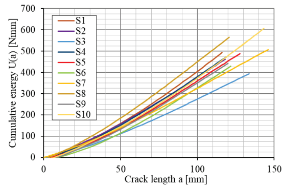
Figure 9: Cumulative energy-crack length curves and (b) R-curves
