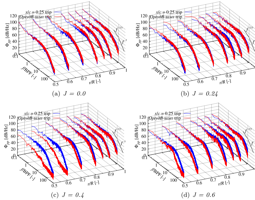
Fig. 8. Wall-pressure power spectral density \Phi_{pp} on the blade suction side at x/c = 0.95 for different spanwise sections. Comparison between x/c = 0.25 and Opty \partial B -BEMT trip computational setups.
