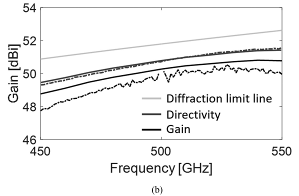
Fig. 19. Lens antenna parameters postprocessed from the coupling measurements. (a) Lens aperture efficiency and (b) gain curve. The solid curves are simulated, whereas the dash-dotted curves are postprocessed from the measurements.
