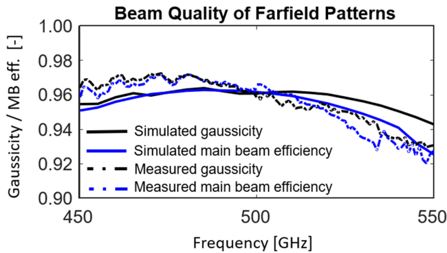
Fig. 16. Beam quality of far-field patterns in terms of Gaussicity (black curves) and main beam efficiency (blue curves). The simulations (solid curves) are compared with the quantities derived from the measured NF-to-FF transformation (dash-dotted curves).
