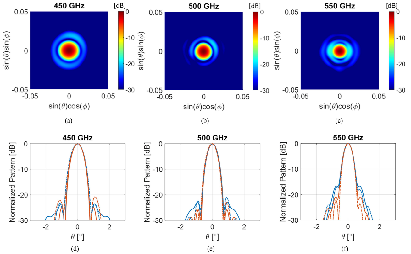
Fig. 15. Far-field lens patterns derived from the measured near field shown in Fig. 14. (a)–(c) 2-D patterns in the uv -coordinates. (d)–(f) Main plane cuts, E-plane (red), and H-plane (blue). Shown are simulated values (solid curves) and the results of the measured NF-to-FF transformation (dashed curves). Results are shown for frequencies 450 GHz (a), (d), 500 GHz (b), (e), and 550 GHz (c), (f).
