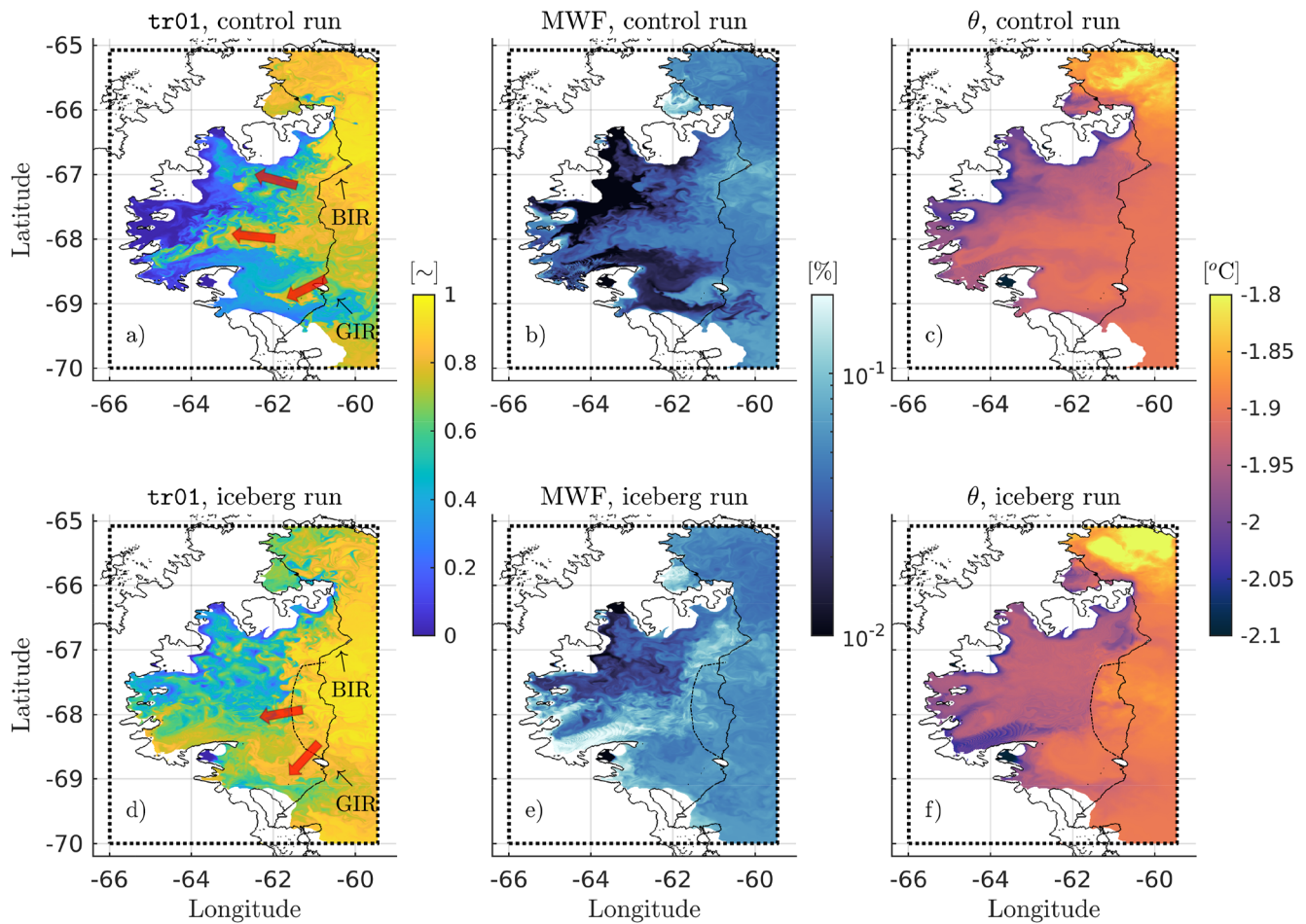
Figure 2. Simulated ocean conditions along the horizontal cross-section corresponding to isopycnal surface 27.90. (a) Concentration of passive tracer \text{tr01} as a snapshot of 1 January 2017. Red arrows show direction of the pathways of \text{tr01} intrusion. (b) Distribution of meltwater fraction (MWF) calculated on the same day. (c) Distribution of potential temperature as an average for December 2016. (d)–(f) are same as (a)–(c) but for the iceberg run.
