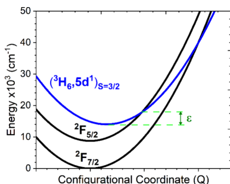
Figure 8. Configurational coordinate diagram revealing the Tm 2+ 2 F 7/2 , 2 F 5/2 , and ( 3 H 6 Sd 1 ) S=3/2 state parabolas. The crossing point between the ( 3 H 6 Sd 1 ) S=3/2 and 2 F 5/2 states exemplifies the quenching process of interband crossing, which is activated at a specific temperature when enough thermal energy \epsilon is available for reaching the crossing point. At an even higher temperature, the crossing point between the ( 3 H 6 Sd 1 ) S=3/2 and 2 F 7/2 ground state will be thermally provoked. 26,27,47,48
