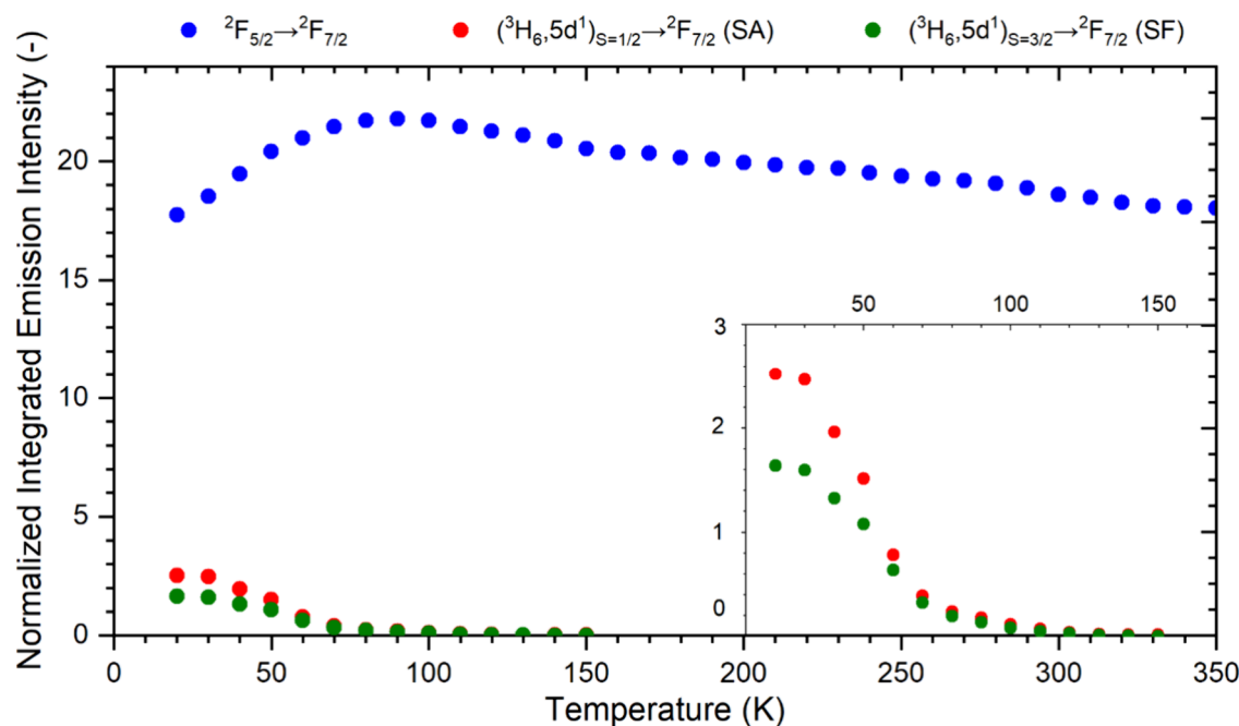
Figure 7. Plot showing the integrated emission intensity of the ^2\text{F}_{5/2} \rightarrow ^2\text{F}_{7/2} (blue), (^3\text{H}_6, ^5\text{d}^1)_{S=1/2} \rightarrow ^2\text{F}_{7/2} (red), and (^3\text{H}_6, ^5\text{d}^1)_{S=3/2} \rightarrow ^2\text{F}_{7/2} (green) emissions after excitation into the (^3\text{H}_6, ^5\text{d}^1)_{S=1/2} levels at 570 nm. The data is normalized and extrapolated on the measured ^2\text{F}_{5/2} \rightarrow ^2\text{F}_{7/2} quantum efficiency at 300 K and corrected for the sensitivity of detection. The inset shows a close-up of the 4\text{f}^{12}5\text{d}^1 \rightarrow 4\text{f}^{13} emissions.
