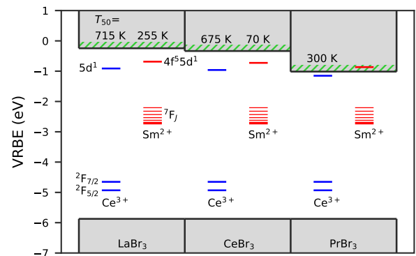
Fig. 10. VRBE diagram for \text{Ce}^{3+} and \text{Sm}^{2+} in \text{LaBr}_3 , \text{CeBr}_3 , and \text{PrBr}_3 . The lowering of the conduction band bottom along the series decreases the quenching temperature of \text{Ce}^{3+} and \text{Sm}^{2+} 4f^{n-1}5d \rightarrow 4f^n emissions.
