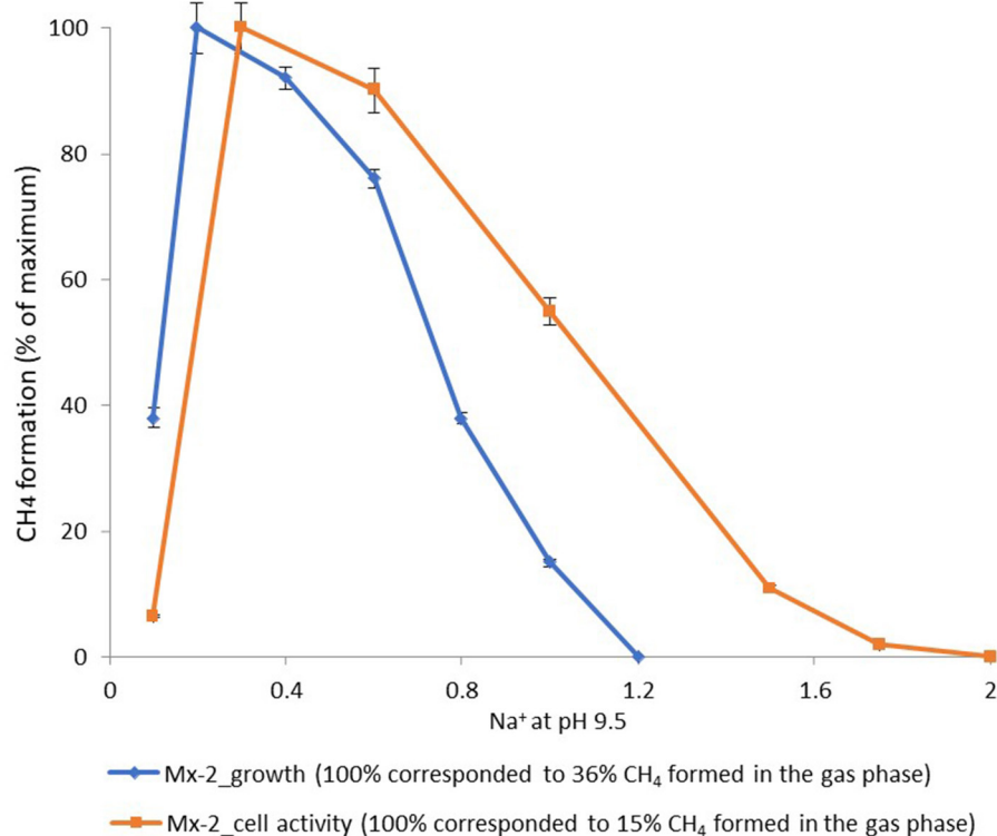
FIGURE 4 Dependence of the methane formation at pH 9.5 by strain Mx on salt concentration of the medium.
