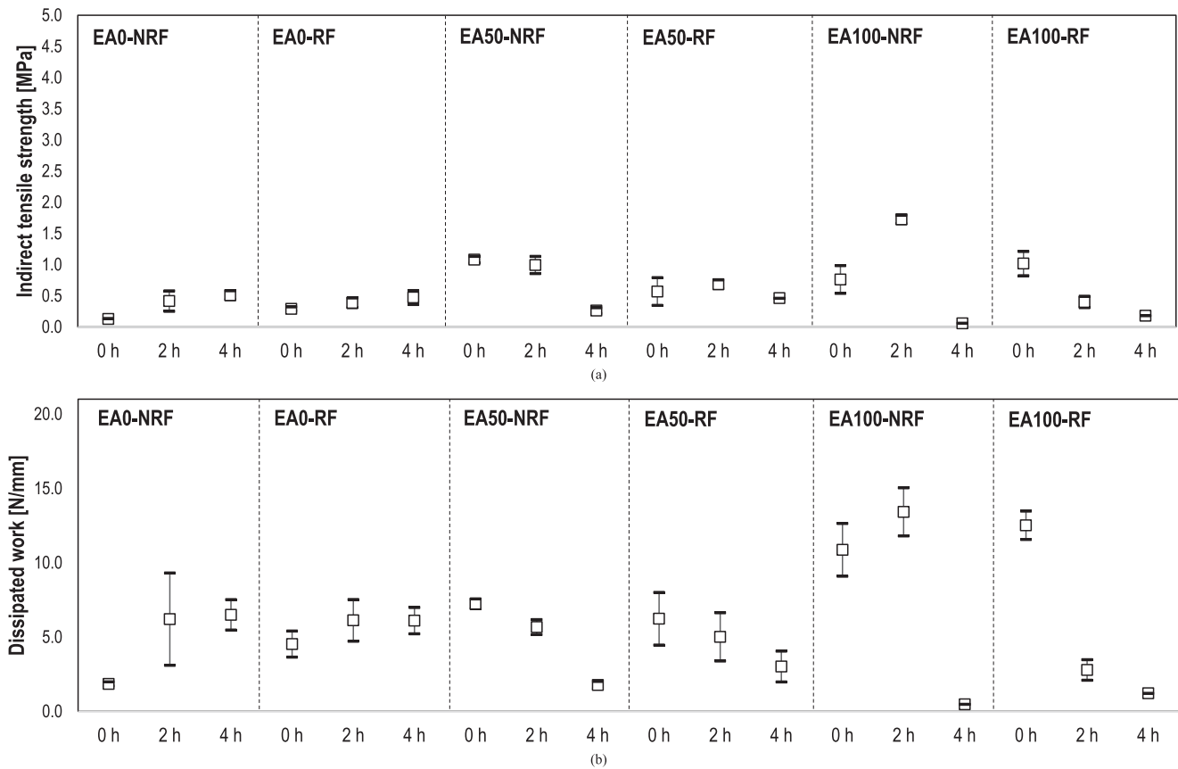
Figure 5. Change of (a) tensile strength and (b) dissipated work of short-term aged materials due to water conditioning.
