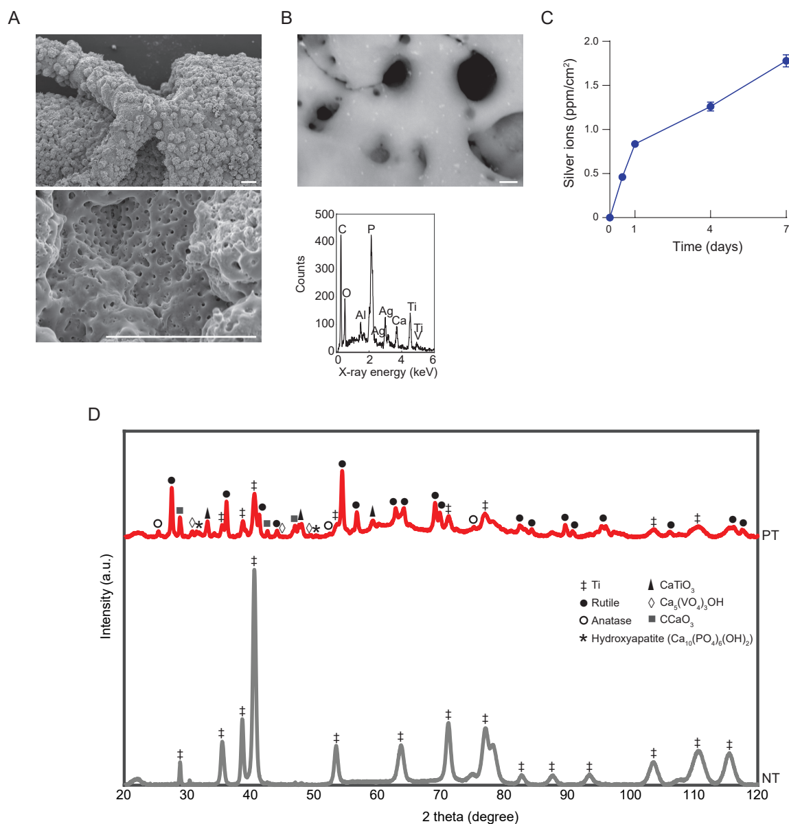
Figure 2. The surface characterization of the PEO-biofunctionalized implants: (A) SEM imaging of the surface of the PT implants, scale bar = 100 \mu m; (B) EDS analysis of the PT-Ag implant surfaces with EDS, scale bar = 1 \mu m; (C) Ag ion release kinetics of the PT-Ag implants ( n = 3 ) over 7 days as measured using ICP-OES; (D) X-ray diffraction spectra of the NT and PT implants.
