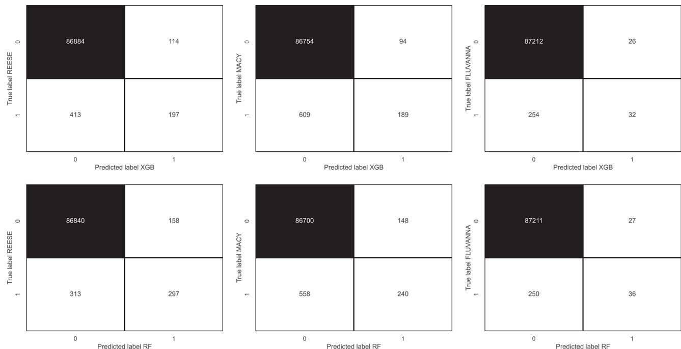
Figure 11. Confusion matrices for extreme wind gust ( W_p > 20 \text{ ms}^{-1} ) prediction. The top and bottom panels represent XGB and RF models, respectively. The left, middle, and right panels correspond to the REESE, MACY, and FLUVANNA stations, respectively.
