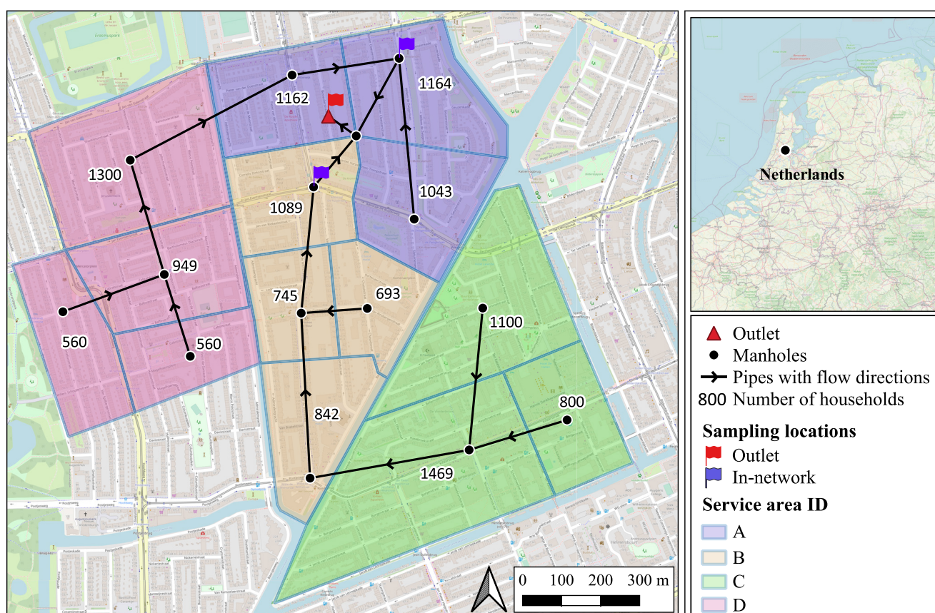
Figure 2. Semi-hypothetical case-study pipe network showing service areas, pipes with flow directions, manholes, sampling locations and an outlet. The service areas are further divided into sub-service areas. The number of households is per sub-service area. The inset map shows the location of the study area within the Netherlands.
