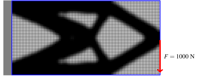
Fig. 2. Cantilever Beam Problem: The blue rectangular domain (50 mm × 100 mm) is the design domain, discretized with a structured mesh of bilinear quad elements. The displacements at the left boundary of the domain are fixed and a point load is applied indicated with a red arrow. The dark layout is the design obtained from compliance minimization.
