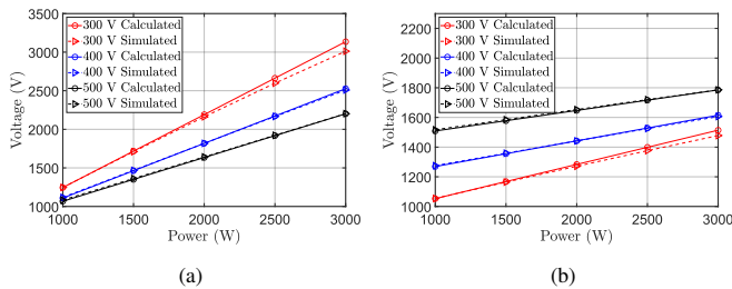
Fig. 6: S-S compensation, M = 105 \mu\text{H} . (a) Peak voltage of primary coil. (b) Peak voltage of secondary coil.
