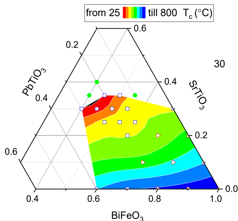
Figure 3. Isothermal map of Curie temperatures with various compositions in BFO-PT-ST ternary system (square—pseudocubic, PC; triangle—rhombohedral, Rh; circle—cubic, C; color scale is linear).
