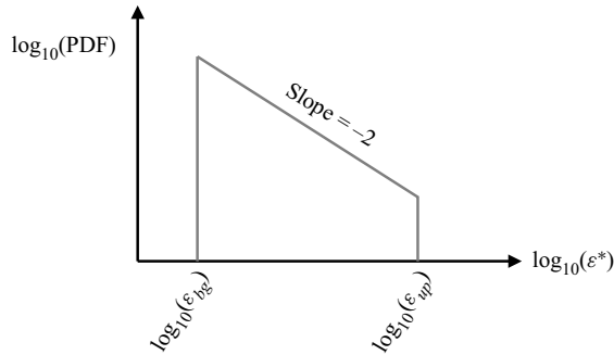
Figure 10. Assumed distribution for the average dissipation \epsilon^* within the layers.
