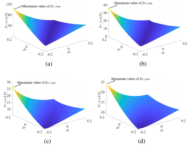
Fig. 8. Value of the peak primary coil current I_{P1\_Peak} under different values of R_E and degree of capacitance drift in Case B. (a) R_E = 5 \Omega . (b) R_E = 25 \Omega . (c) R_E = 45 \Omega . (d) R_E = 65 \Omega .
