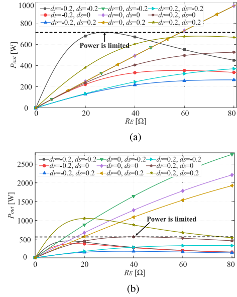
Fig. 5. Output power P_{out} versus the equivalent load resistance R_E under parameter deviations. (a) Case A. (b) Case B.
