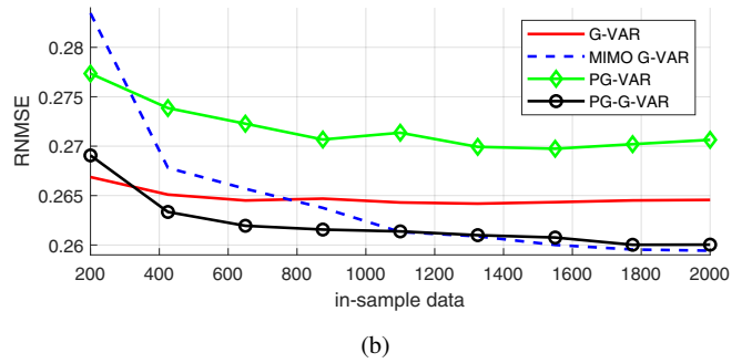
Fig. 1: RNMSE versus the amount of in-sample data for the different graph-based models. Where at (a) the results are shown when the initial feature graph is used and at (b) the joint estimation method is used to find the optimal feature edge weights.
