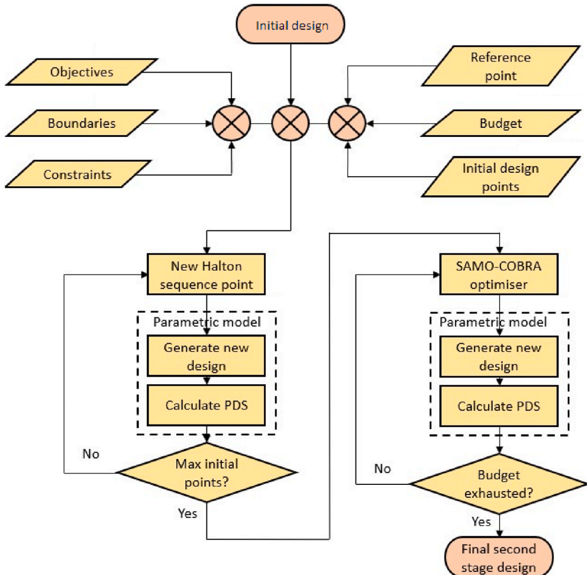
Fig. 1. Flowchart of the optimisation framework proposed.
