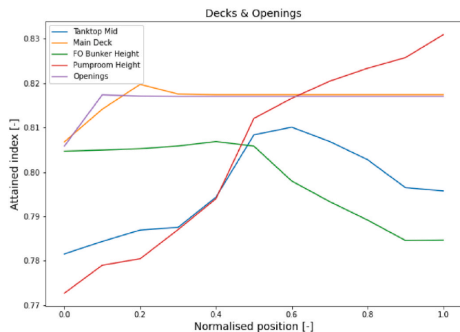
Fig. 18. Sensitivity in the normalised range of the decks and openings concerning the attained index A.
