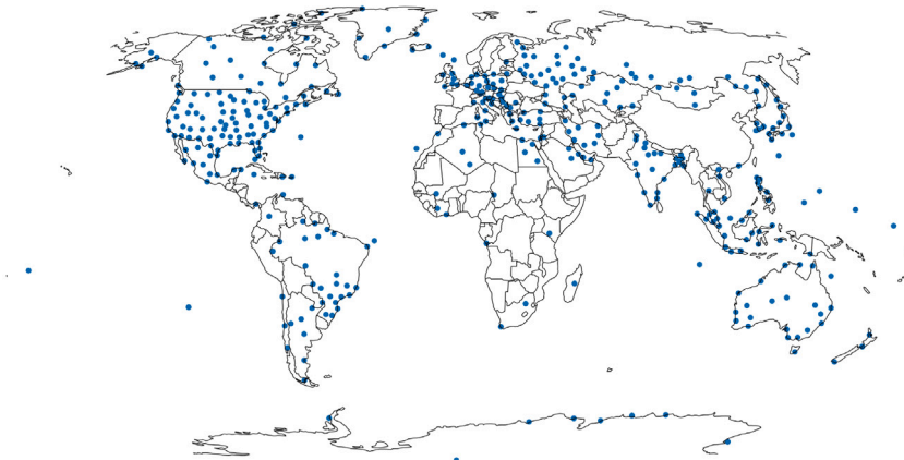
(b) IGRA station locations used in this research
