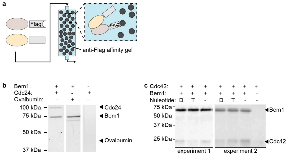
Figure 4.5. Bem1-Cdc24 and Bem1-Cdc42 binding. (a) Schematic illustration of Flag-pulldown experiments. (b) SDS-PAGE of elution fractions of Flag-pulldown experiments with H-Bem1-F, Cdc24-H, and Ovalbumin. (c) Anti-His Western Blots of elution fractions of two Flag-pulldown experiments with H-Bem1-F and S-Cdc42-H preloaded with no nucleotide, GDP (D), or GTP \gamma S (T).
