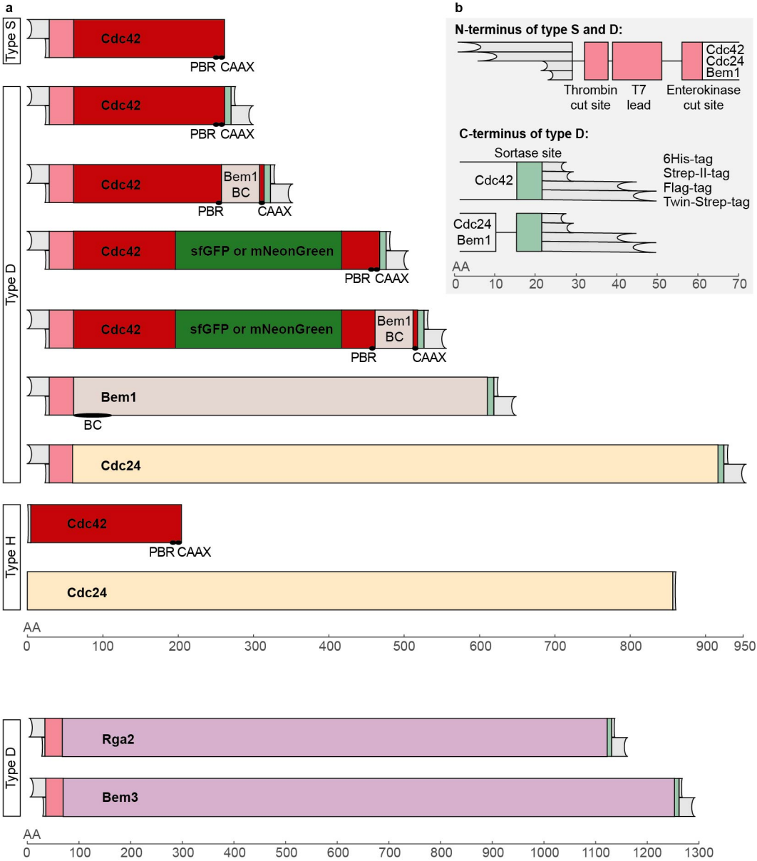
Figure 2.1. Schematic overview of the protein constructs. (a) Illustration of the general size and outline of double-tagged (type D) and single-tagged constructs (type S) and of constructs to which only a single 6His-tag got added N- or C-terminally (type H). Additionally, protein domains of special interest are annotated. (b) Zoom-in of the N- and C-terminal tag regions from type S and D and illustration of the size difference of the purification tags. Please note, the T7 lead illustrated here is also commonly known as the T7 tag. All constructs are drawn roughly up to scale, in terms of their number of amino acids (AA). An overview of the specific constructs is given in Tab. 2.3.
