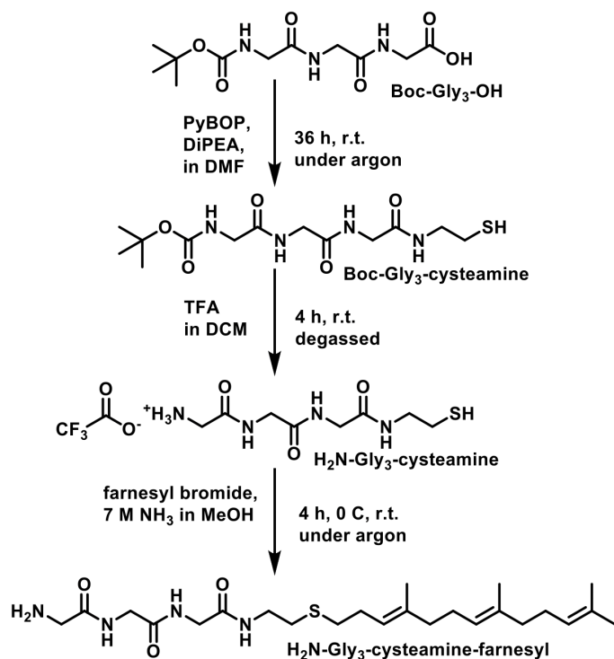
Figure 2.3. General synthetic procedure going from Boc-Triglycine to the C-terminally farnesylated triglycine derivative ('farnesyl peptide'). Abbreviations: r.t.: room temperature.
