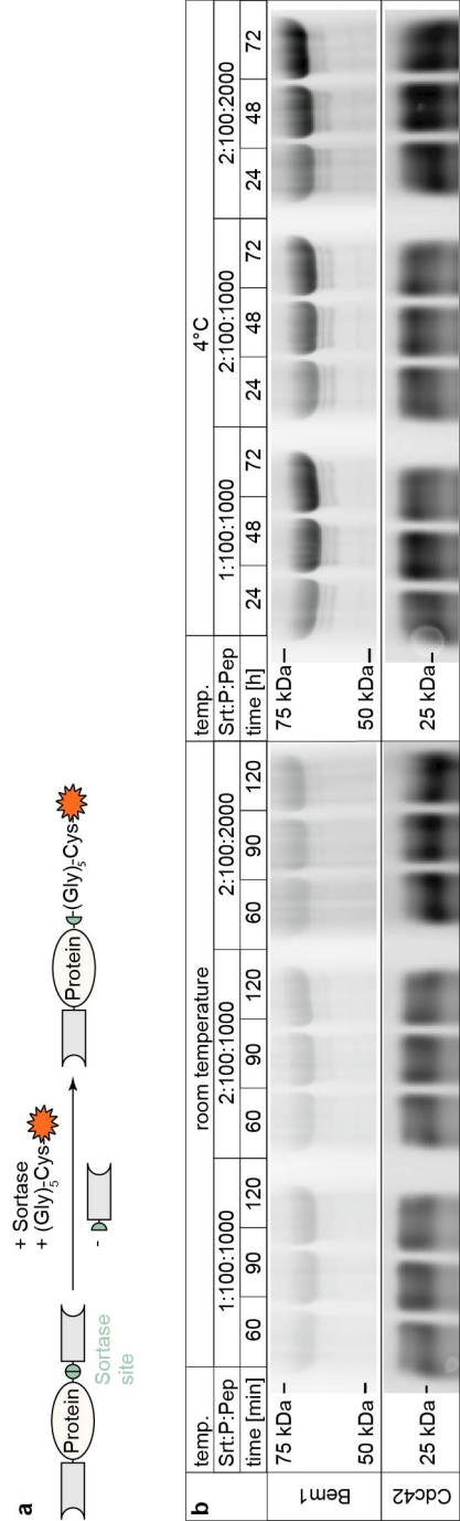
Figure 5.2. Sortase-mediated labelling of Cdc42 and Bem1 with Alexa488- and farnesyl-peptide. (a) Schematic illustration of the Sortase-mediated labelling reaction of double-tagged protein (Cdc42 or Bem1) with Alexa-peptide. (b) Condition screen of the labelling reaction of Bem1 (S-Bem1-H, 70 kDa) or Cdc42 (S-Cdc42-H, 29 kDa) with Alexa488 peptide, using stated temperatures, Sortase : protein : peptide (Srt:P:Pep) ratios, and incubation times. SDS-Page of the Alexa488-signal are shown.
