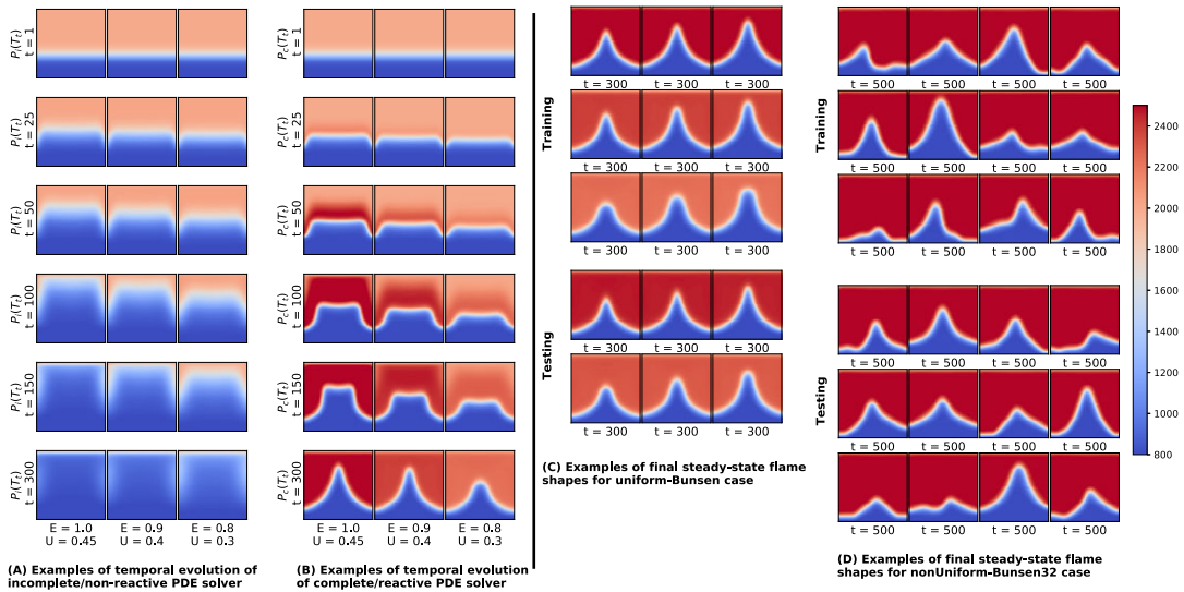
Figure 6. Instances of temporal evolution of (A) incomplete PDE solver; (B) complete PDE solver for different operating conditions. (C) Snapshot of complete PDE solver at t=300 for all training and testing datasets of the uniform-Bunsen case. (D) Snapshot of complete PDE solver at t=500 for all training and testing datasets of the nonUniform-Bunsen32 case.
