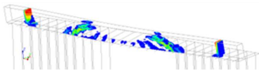
Figure 6: Cracks in a quay wall associated with foundation failure and due to passage of heavy vehicular traffic as observed from numerical simulations reported in [9].
