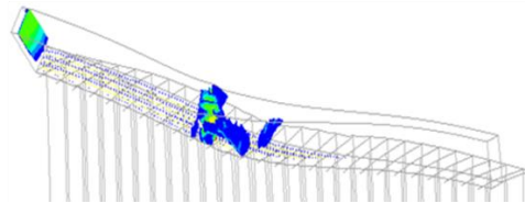
Figure 6: Cracks in a quay wall associated with foundation failure and due to passage of heavy vehicular traffic as observed from numerical simulations reported in [9].
