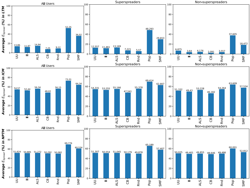
Fig. 4. Average expected spread for each of RA, for all users, superspreaders (defined by \theta = 60\% ), and non-superspreaders in the POLITIFACT FAKE NEWS NET DATASET according to the Linear Threshold model (LTM—top row), Independent Cascade model (ICM—middle row), and the Node Profile Threshold Model (NPTM—bottom row).
