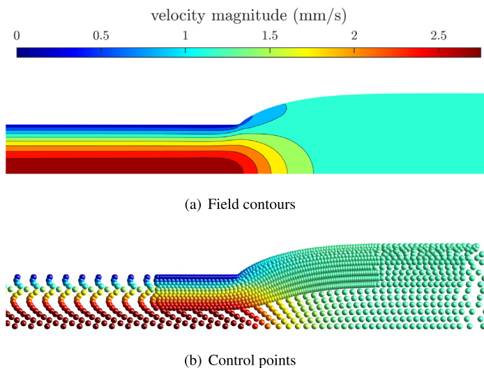
Fig. 21. Velocity magnitude during steady state ( t = 7.50 s) in the exit region.
