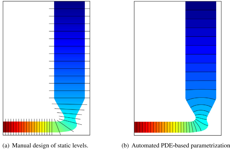
Fig. 11. Schematics of the old (a) and new (b) concept for the undistorted parametrization of physical space w.r.t. \xi . Colors indicate values of \xi . (For interpretation of the references to color in this figure legend, the reader is referred to the web version of this article.)
