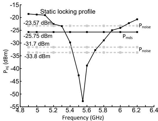
Fig. 4.15: Static locking profile and minimum input power ( P_{mds} ) for locking to f_c=5.55 GHz f_m=250 MHz and \beta=1 . The integrated noise levels applied are annotated.
