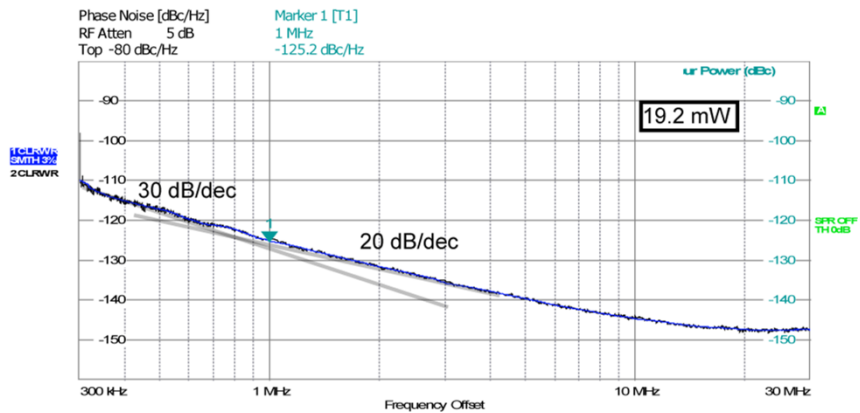
Fig. 6.11: Phase noise measured at 25.8 plot (a) and 19.2mW (b), when operated from 1.2V. The GSM/DCS Mobile (MS) and Base station (BTS) specifications are normalized to the 3.92 GHz carrier frequency.
