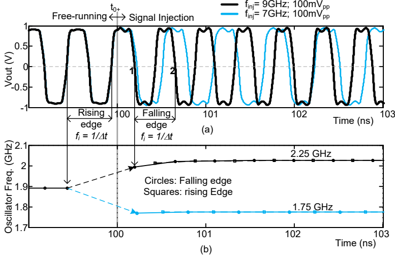
Fig. 3.4: Simulated locking response for f_{inj} of 9 and 7 GHz applied at 100 ns (a) time-domain simulation of the output voltage, and (b) instantaneous frequency vs. time.
