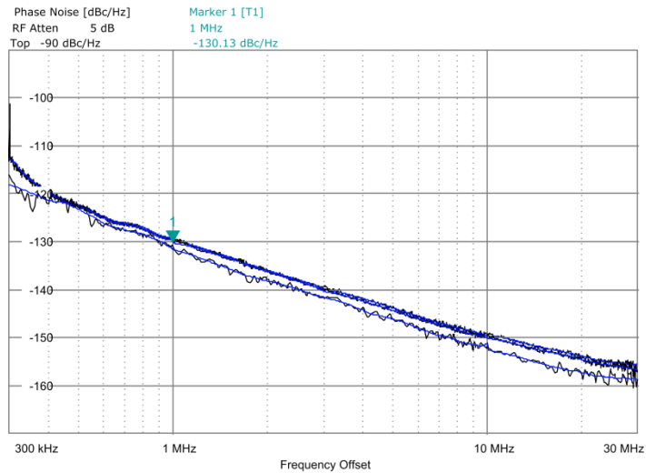
Fig. 6.14: Phase noise measured at mid-band and tuning range extremes. The variation across the tuning range at 1 MHz offset is ~1.6 dB.
