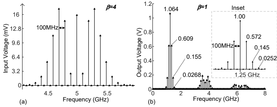
Fig. 3.5: Transformation of modulation index. (a) Input 80mV pp FM signal with f_c = 5 GHz, f_m = 100 MHz and \beta = 4 , and (b) differential output of the locked-in oscillator. FM deviation is divided by 4, and the input \beta of 4 is translated to 1.
