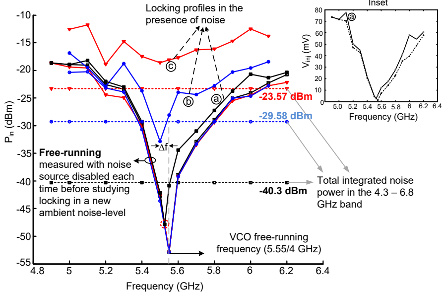
Fig. 4.13: Locking profile measured before and after applying different levels of integrated noise power to the locking signal. The oscillator's f_0 is set mid-band at 5.55 GHz/4. The free-running profile and curve 'a' are shown in mV scale in the inset.
