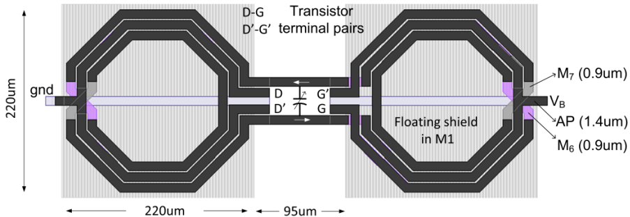
Fig. 6.8: Layout view of the two-transformer core.
