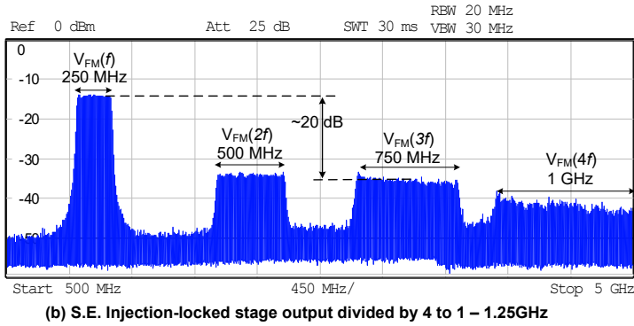
Fig. 4.4: Division of FM deviation. (a) 4–5 GHz bandwidth input FM, (b) Input bandwidth is divided down by a factor of 4 (1.00–1.25 GHz).
