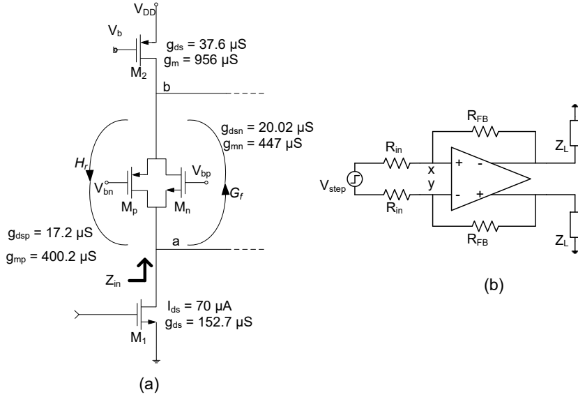
Fig. 5.7: Monticelli-cell analysis and operating point values used to evaluate eqns. 5.22 to 5.24, and (b) fully differential shunt-feedback configuration.
