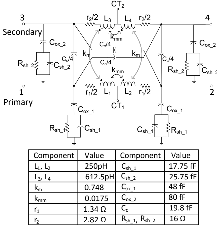
Fig. 6.3: Lumped equivalent model of the 1:2 feedback transformers shown in Fig. 6.1.
