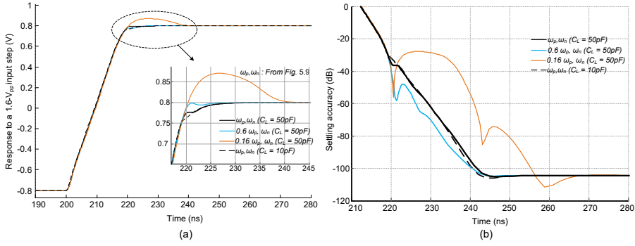
Fig. 5.10: Step-response showing the effect of the slow settling component for varying loop-bandwidths when the load equals 50 \Omega \parallel 50 pF.
