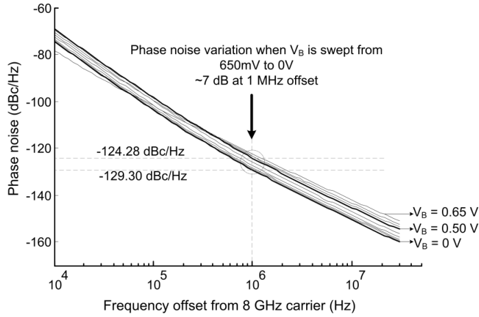
Fig. 6.6: Spectre-RF™ simulation of PN at 8 GHz, for V_B varied from 650 mV to 0 V. Phase noise improves by 5.1 dB at 1 MHz offset for V_B = 500 mV (23.4 mA) and 0 V (33.5 mA).
