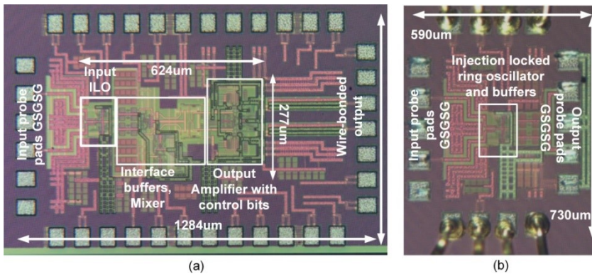
Fig. 4.1: 65nm CMOS chip micrograph of: (a) the IF demodulator with 624 \times 277\text{-}\mu\text{m}^2 core area, and (b) the stand-alone injection-locking oscillator.
