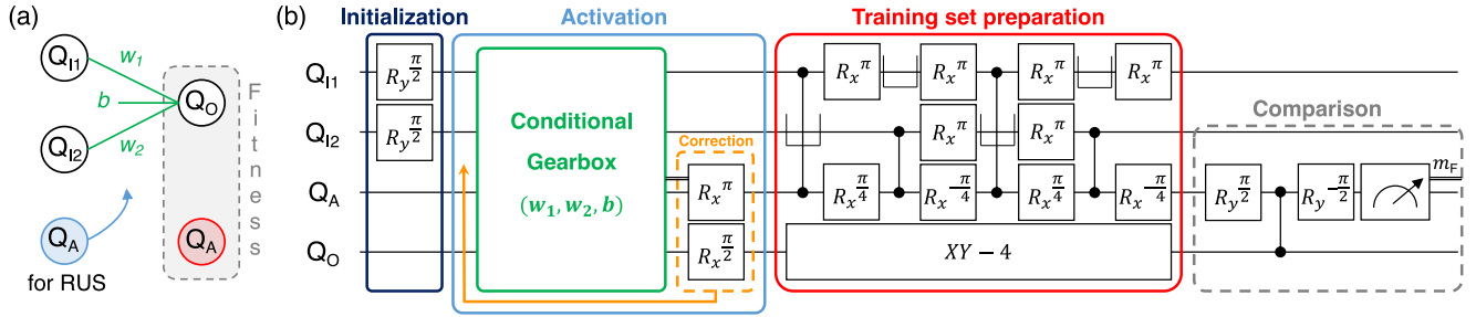
Fig. 4 Quantum neural network using the repeat-until-success conditional gearbox circuit. a Schematic representation of simplest feedforward network, highlighting the role played by parameters ( w_1, w_2, b ) in weighing the sum of input signals, before the result is passed through a non-linear activation function. Q_{I1} and Q_{I2} are input nodes, Q_O is the output node and Q_A is an ancilla used first within the RUS circuit and then as expected output for the training set. b Quantum circuit for a 3-neuron feedforward network. This circuit is divided into four steps. Input ( Q_{I1}, Q_{I2} ) preparation into maximal superposition; threshold activation into Q_O using RUS conditional gearbox circuit with ( w_1, w_2, b ); unitary encoding of Boolean function (AND, in this case) using oracle; and comparison of Q_A with Q_O . XY-4 specifies an error mitigation sequence 38 applied during measurement and the symbol \sqcup denotes parking of spectator qubit Q_{I2} ( Q_{I1} ) during CZ( Q_A, Q_{I1} ) (CZ( Q_A, Q_{I2} )) gates [Supplementary Materials].
