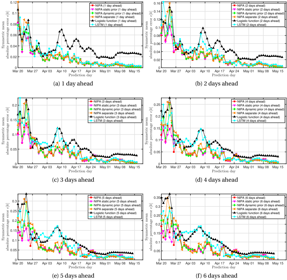
Figure 7.5: The prediction accuracy for the situation in the Netherlands. The subplots show the prediction accuracy (a) 1 day ahead, (b) 2 days ahead, (c) 3 days ahead, (d) 4 days ahead, (e) 5 days ahead and (f) 6 days ahead.
