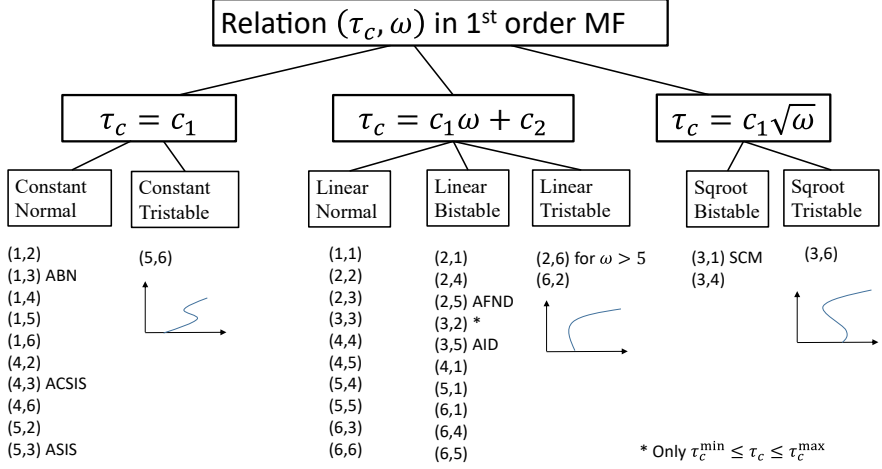
Figure D.1: The relation between the epidemic threshold \tau_c and the effective link-breaking rate \omega under the first-order mean-field approximation for all 36 instances of the G-ASIS model. We categorise the instances under three main pillars: Constant (left), Linear (middle) and Other (right). Within each pillar, several further distinctions are given. Each G-ASIS instance is specified by the pair (i, j) , where i specifies the link-breaking rule and j represents the link-creation rule. The number 1 represents the link-updating rule from the 1st row from Table 4.1, the number 2 the second row, etc.
