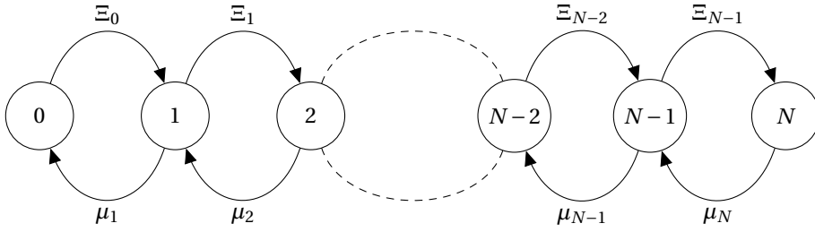
Figure 2.1: The Markov chain \mathcal{M} of the \varepsilon -SIS process on the complete graph K_N with N nodes is a finite birth and death process with birth rate \Xi_k = (\beta k + \varepsilon)(N - k) and death rate \mu_k = \delta k . The state M = 0, \dots, N of the Markov chain denotes the number of infected nodes in the graph. Furthermore, \beta is the infection rate, \delta the curing rate and \varepsilon the self-infection rate.
