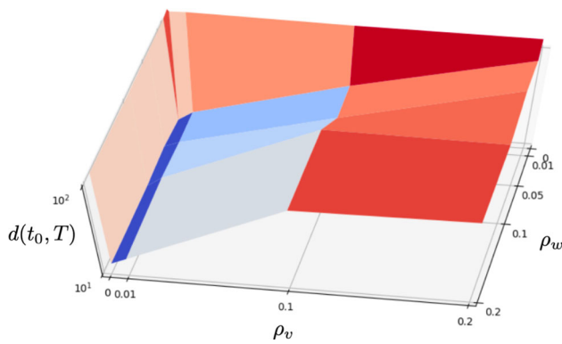
Fig. 5 Results for combinations of \rho values
