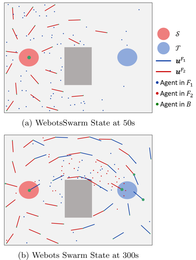
Fig. 1 Webots swarm state with obstacle
