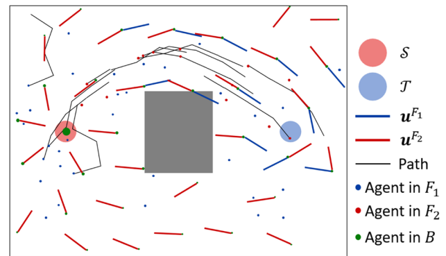
(a) Adapting swarm after 100s.
