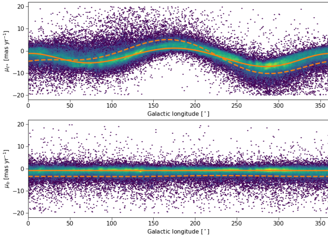
Fig. 32. Proper motions in Galactic longitude ( top ) and latitude ( bottom ) as a function of Galactic longitude for the sample of 385 423 B-stars described in the text. The lines show the proper motions predicted from the rotation curve model parameters resulting from the fit to the data for stars at 500 pc (dashed line) and 2000 pc from the Sun (solid line, close to the median distance of stars in the sample).
