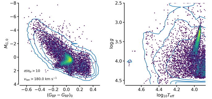
Fig. 5. Distribution of the parameters of the OBA sample with \varpi/\sigma_\varpi > 10 and v_{\text{tan}} > 180 \text{ km s}^{-1} . Left : observational HR diagram. Right : Kiel diagram. The contours indicate the distribution of the full sample. The colour code indicates the density of sources satisfying the above criteria.
