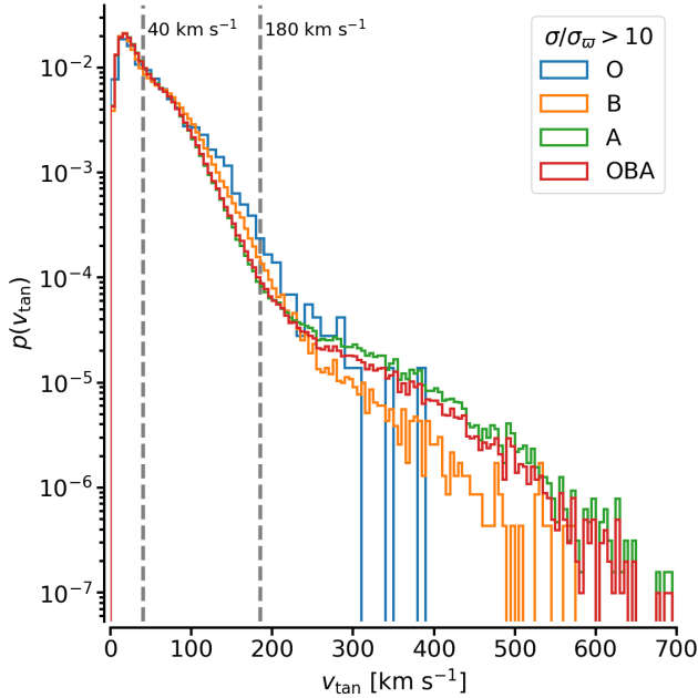
Fig. 3. Histogram of tangential velocities of the stars in the OBA sample with \varpi/\sigma_\varpi > 10 . The combined OBA star sample is shown as well as the individual O, B, and A star samples (based on the classifications from the ESP-HS module). The limits in tangential velocity separating the thin disc, thick disc, and halo populations are shown as vertical dashed lines.
