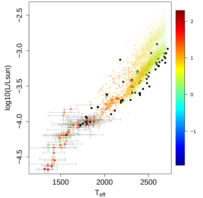
Fig. 18. Bolometric luminosities of candidate UCDs in the Gaia golden sample. The colour code indicates the logarithm of the VOSA fit \chi^2 values, squares represent the data points in Table 1 of Dieterich et al. (2014), and black asterisks denote unresolved binaries therein.
