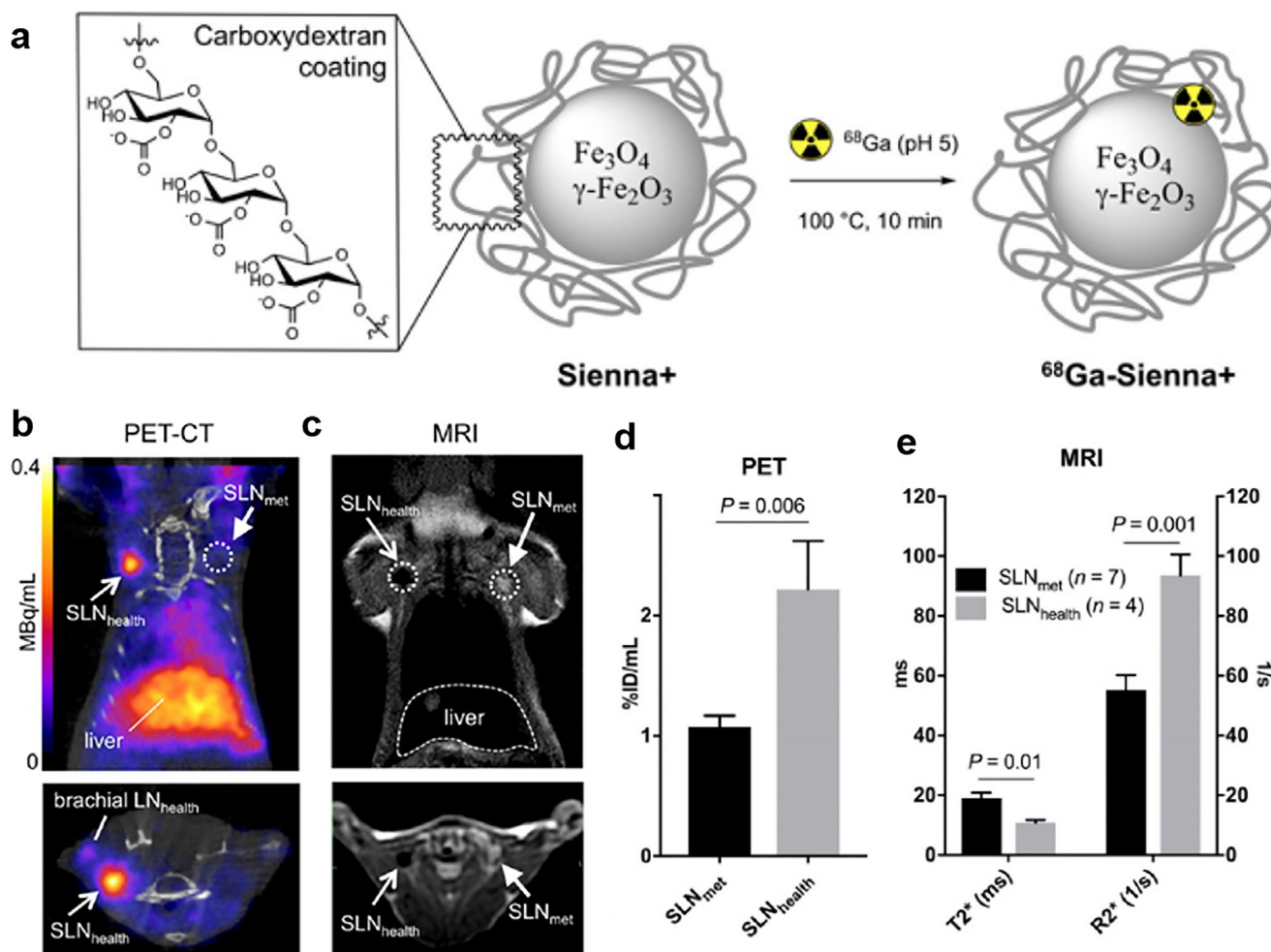
Figure 2. a) ^{68}\text{Ga} -radiolabelling of Sienna+; In vivo imaging in the 3E.Δ.NT metastatic breast cancer model: b) coronal and transversal PET-CT images for the mouse showing uptake of ^{68}\text{Ga} -Sienna+ in SLN health (open arrowhead), but not in SLN met. Note that, for clarity, the injection site and corresponding PET signal is not shown; c) coronal and transversal MRI images (T2-weighted 3D turbo spin echo) of the same mouse showing the uptake of ^{68}\text{Ga} -Sienna+ in SLN health, but not in SLN met that appear bright and enlarged; ^{68}\text{Ga} -Sienna+ uptake quantification (mean \pm SEM) in SLN met and SLN health by d) PET and e) MRI. Adapted with permission. [22] Copyright 2019, Ivyspring International Publisher.
