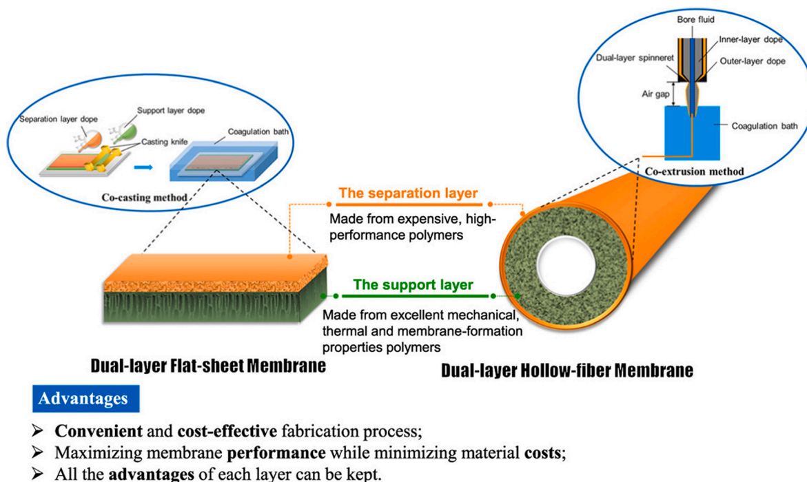
Fig. 8. Conceptual schematic of dual-layer flat-sheet and hollow fiber membranes and fabrication methods. Reprinted with permission from Ref.196, Copyright 2018, Elsevier.
