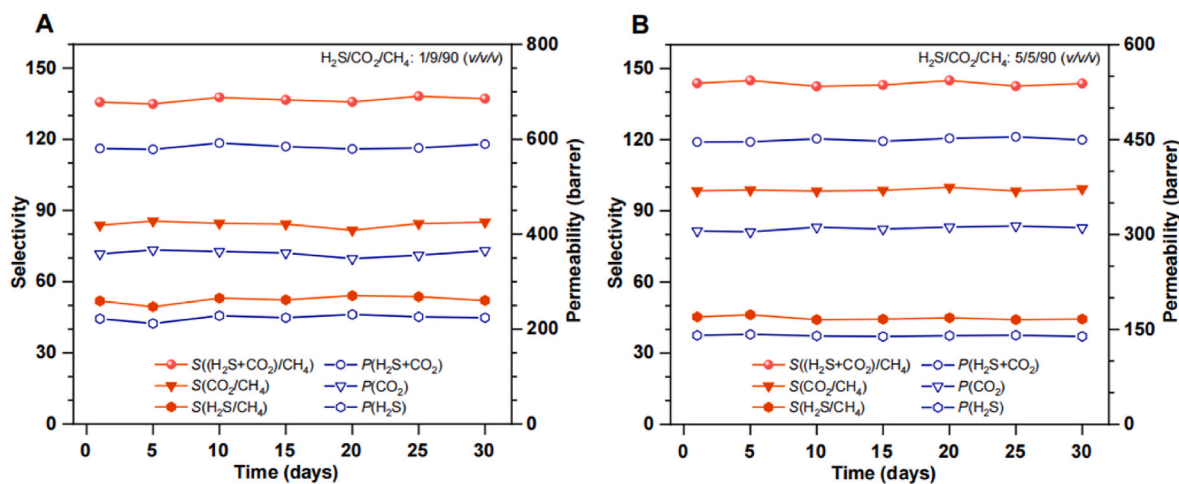
Fig. 6. (A and B) Membrane stability under different H 2 S concentration, (A) H 2 S/CO 2 /CH 4 : 1/9/90; (B) H 2 S/CO 2 /CH 4 : 5/5/90. Robust H 2 S/CO 2 /CH 4 separation properties of (001)-AlFIVE(59.6)/6FDA-DAM-DAT membrane for at least 30 days. Feed pressure at 10 bar and 35 °C. Reproduced with permission from ref. 141, Copyright 2022, Science.
