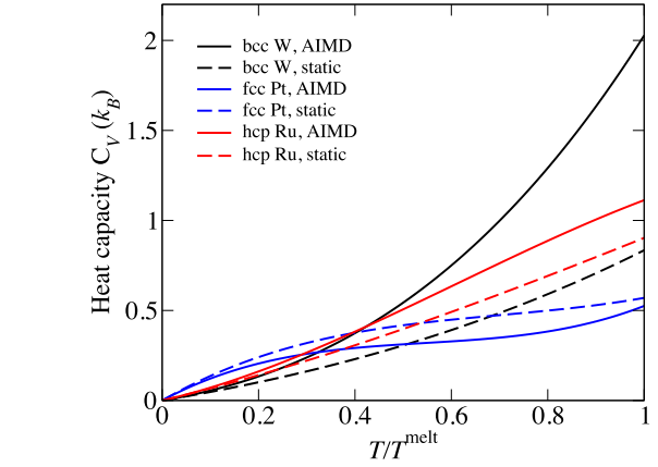
FIG. 10. Temperature dependence of the constant volume electronic heat capacity for bcc W (black), fcc Pt (blue), hcp Ru (red) with (solid lines) and without (dashed lines) the impact of vibrations. To obtain an accurate heat capacity from the coarse set of free energies (see Fig. 8), we used a physically motivated fit as introduced in Ref. [25] with a second-order polynomial for the energy independent electronic density of states. For consistency, the same fit was used to obtain the temperature dependence of the ideal lattice SCF heat capacities (dashed lines). The temperature axis has been normalized by the respective melting temperature.
